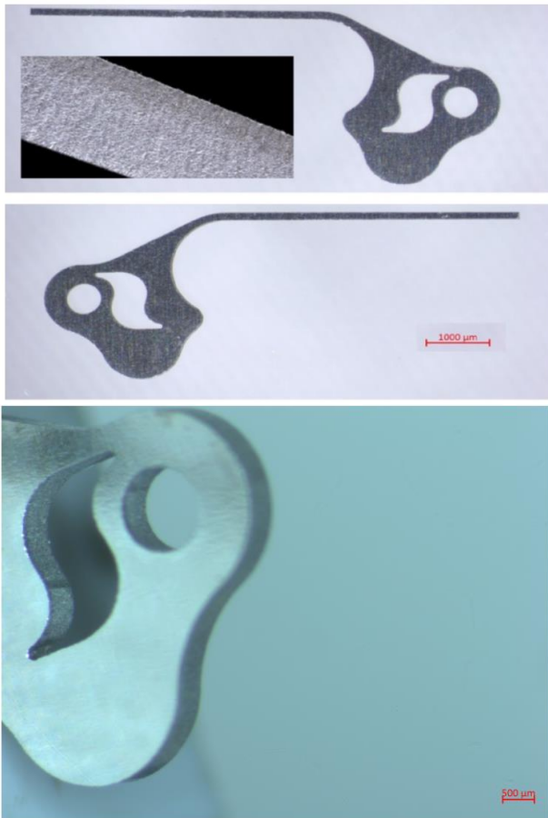
Figure 2 : Ressort.
