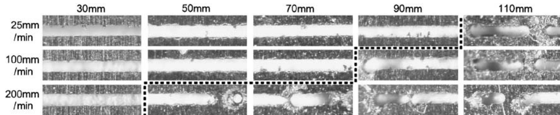
Fig. 10 0.1 mm stainless steel cut at various distances and speeds at 0° incidence
