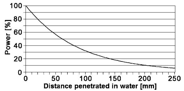
Fig. 3 The remaining laser power after water absorption
