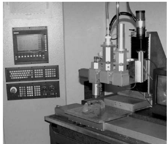
Fig. 4 The water jet guided laser at ITW-Chemnitz
